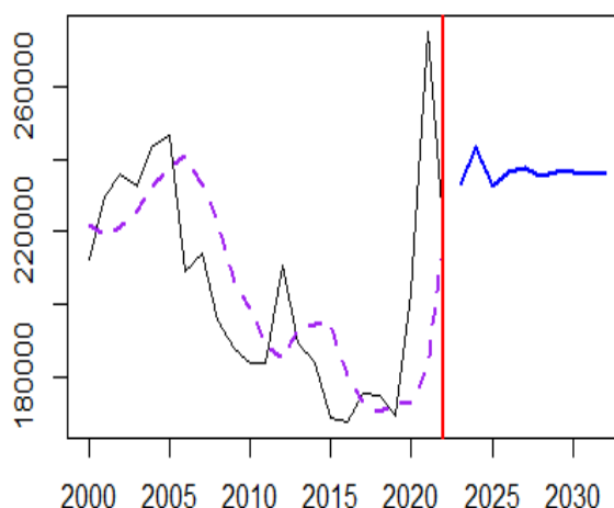
Forecast from SMA(3) with Normal distribution
